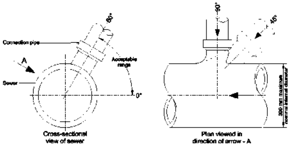
Figure B26: Connections to sewer
