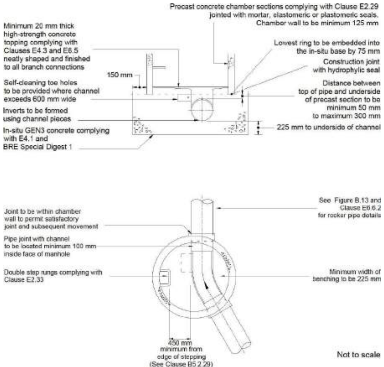
Figure B10: Alternative base detail for Type A and Type B manholes without concrete surround
