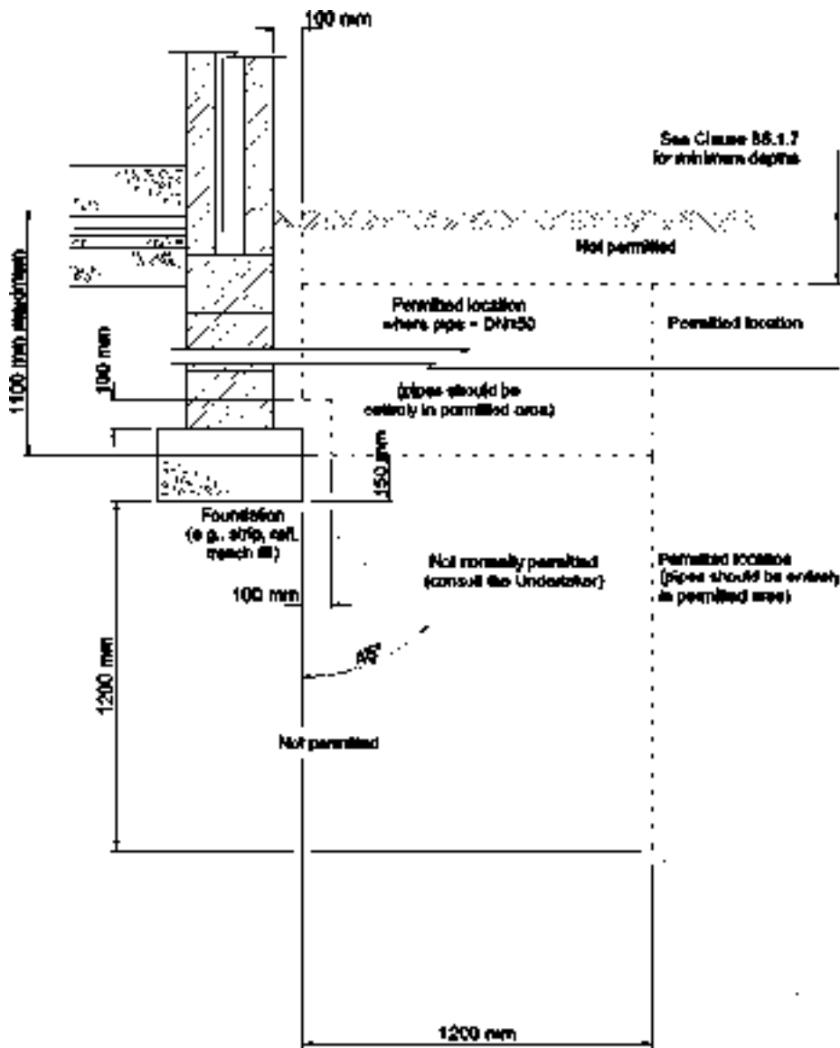
Figure B1: Illustration of the permitted locations of adoptable sewers and lateral drains in proximity to buildings
