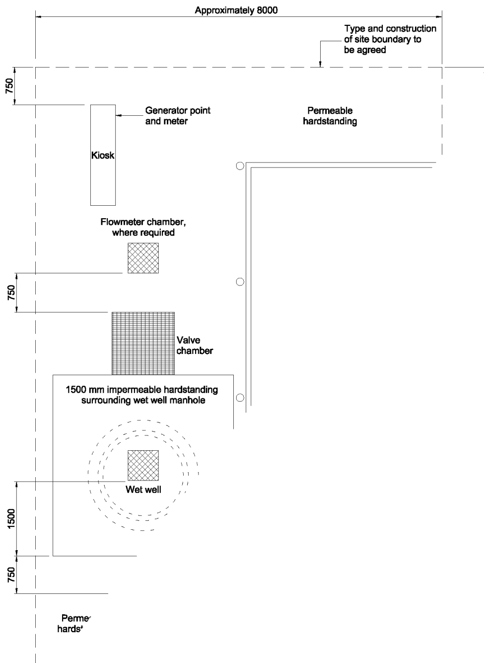
Figure D3: Typical Type 3 pumping station layout
