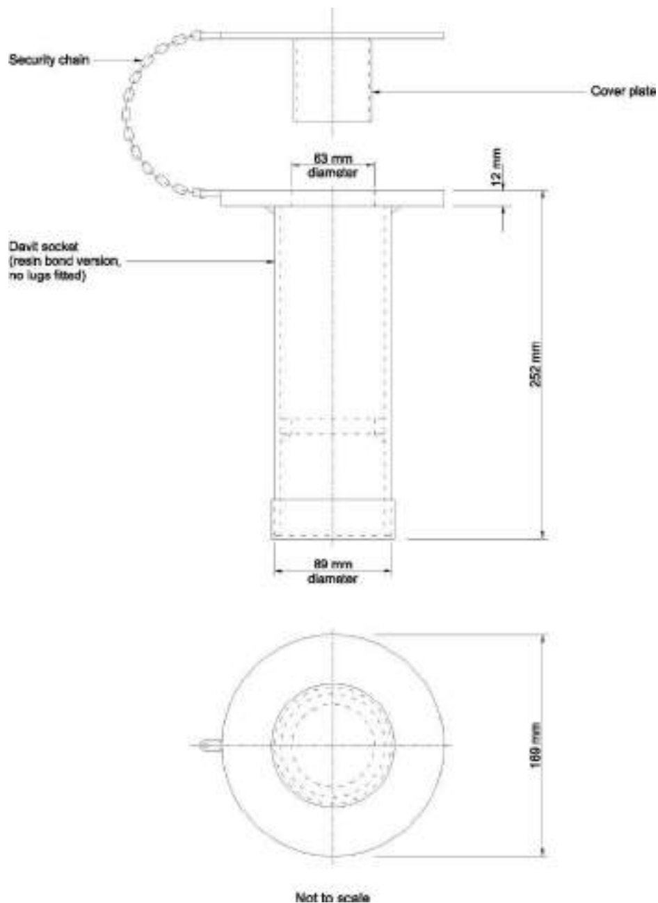
Figure D1: Standard flush mount davit socket
