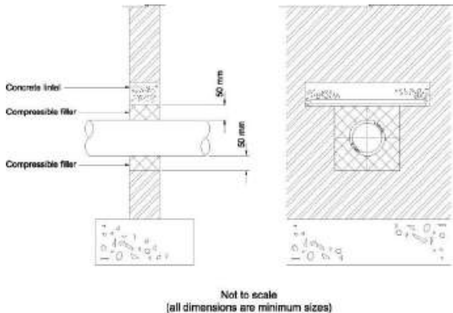
Figure B29: Protection of pipes penetrating single leaf boundary walls
