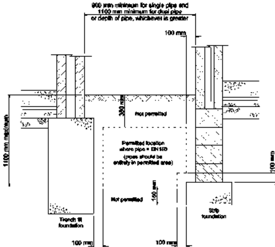
Figure B2: Illustration of the permitted location of small diameter adoptable sewers and lateral drains between buildings
